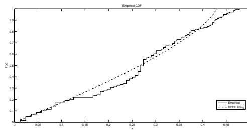
Fig. 11. Fitted GPDE with PWM via SM.
