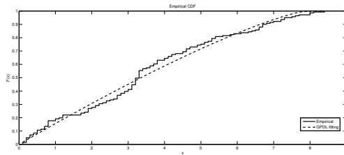
Fig. 8. Fitted GPDFL with PWM via SM.
