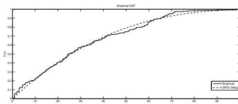
Fig. 1. Fitted GPDL with PWM.
