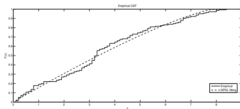
Fig. 10. Fitted GPDF with PWM via SM.
