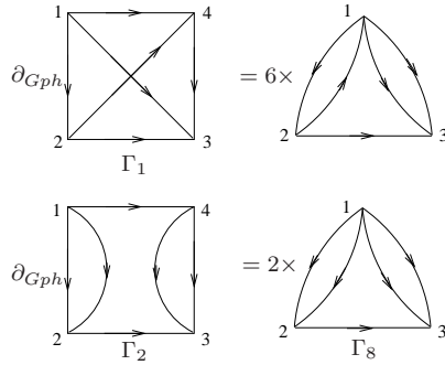
FIG. 3: Graph differential
