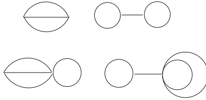
FIG. 1: Symmetry factor for the graphs are 12, 8, 12, 16 respectively
