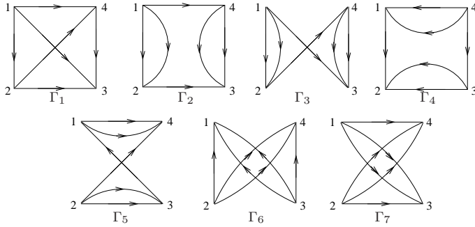
FIG. 4: Wick's contraction
