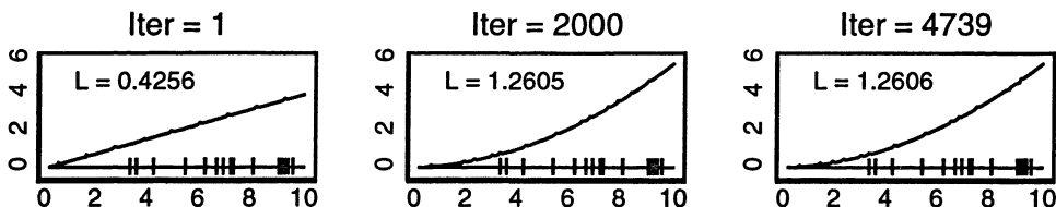
Fig. 1. Three steps of calculating the intensity as a single spline.
