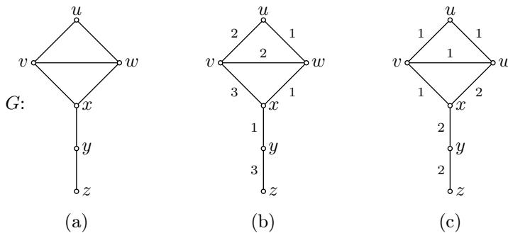
Figure 1. A detectable coloring of a graph
