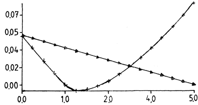
Fig. 7.10. \Gamma_C(\alpha_h^0) ( \Delta ) and \Gamma_C(\alpha_h^6) (+).
