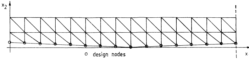
Fig. 7.1. Triangulation of \Omega_h(\alpha_h) for some \alpha_h \in \mathcal{Q}_{\text{ad}}^h .
