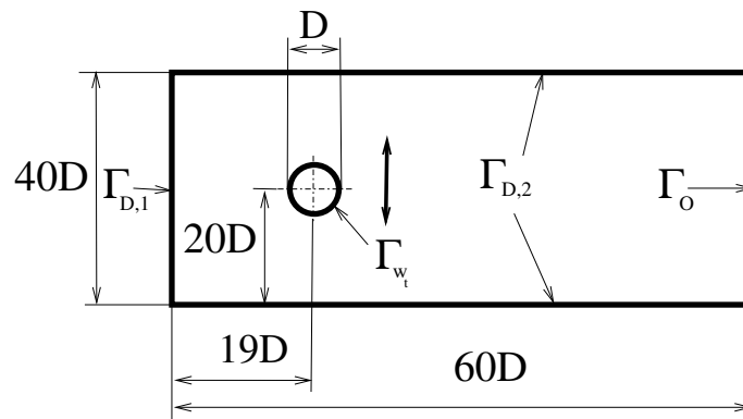
Figure 1: Fluid domain \Omega_{\text{ref}} of the considered benchmark of flow around a movable cylinder, represented by interface \Gamma_{W_t} . Boundary \Gamma_D consists of two parts \Gamma_{D,1} and \Gamma_{D,2} , where \Gamma_{D,1} represents inlet and \Gamma_{D,2} represents walls.
