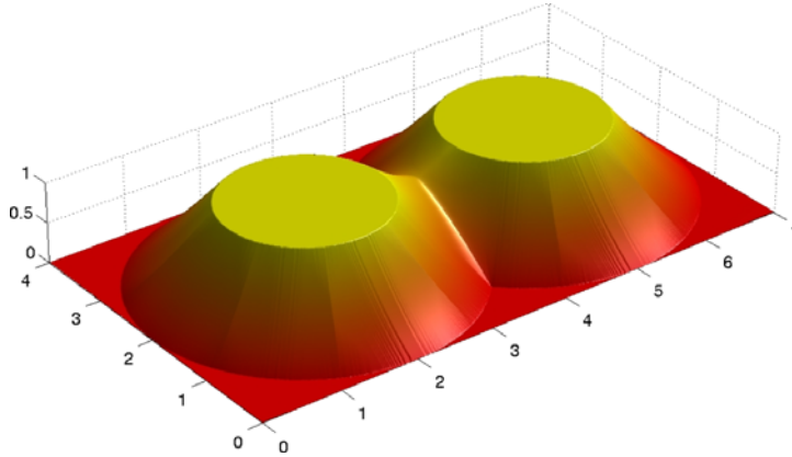
Figure 1.1. Graph of the function U_\infty(x) .
