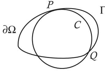
Figure 2.1. An impossible situation.
