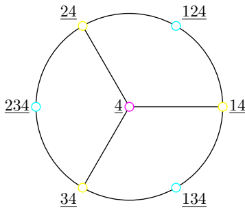
Figure 2. South Polar Cask for d = 3 .
