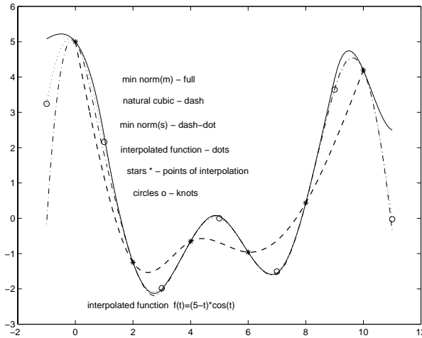
Figure 2. Hermite spline interpolants.
