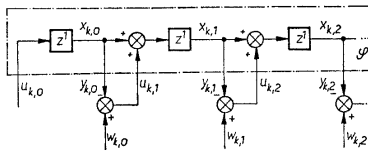
Fig. 15. The optimal control system in Example 5.8.
