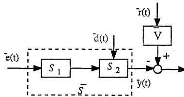
Fig. 8. An open-loop connection.
