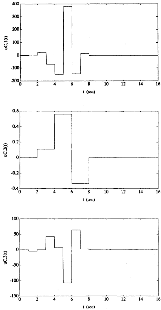
Fig. 5. The components of the continuous-time control input response u_C(t) of S_C for \beta = \beta_0 , z(0) = [0 \ -2]' , x(0) = [1 \ -0.5 \ 2]' , w_C(0) = 0 and w_D(0) = 0 .
