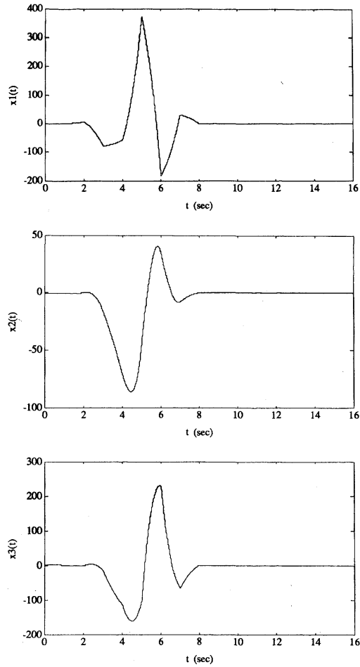
Fig. 3. The components of the continuous-time state response x(t) of the plant \mathcal{P} for \beta = \beta_0 , z(0) = 0 , x(0) = [1 \ -0.5 \ 2]' , w_C(0) = 0 and w_D(0) = 0 .
