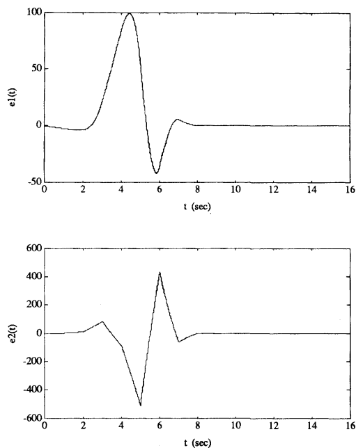
Fig. 4. The components of the continuous-time error response for \beta = \beta_0 , z(0) = [0 \ -2]' , x(0) = [1 \ -0.5 \ 2]' , w_C(0) = 0 and w_D(0) = 0 .
