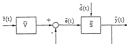
Fig. 7. The feedback system \bar{\Sigma} .
