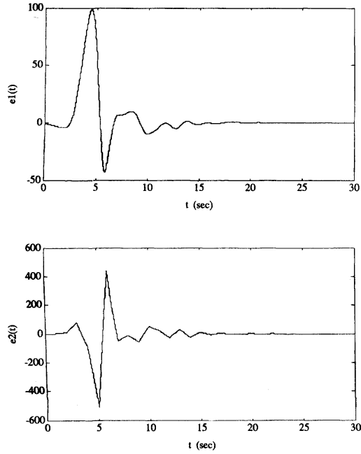
Fig. 6. The components of the continuous-time error response for \beta = [0.5003 \ -0.0008]' , z(0) = [0 \ -2]' , x(0) = [1 \ -0.5 \ 2]' , w_C(0) = 0 and w_D(0) = 0 .
