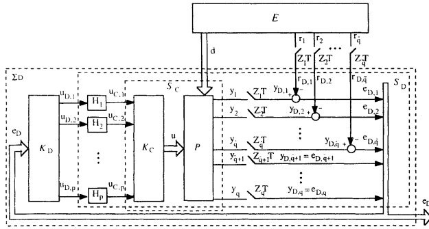
Fig. 1. Structure of the hybrid multirate sampled-data control system.
