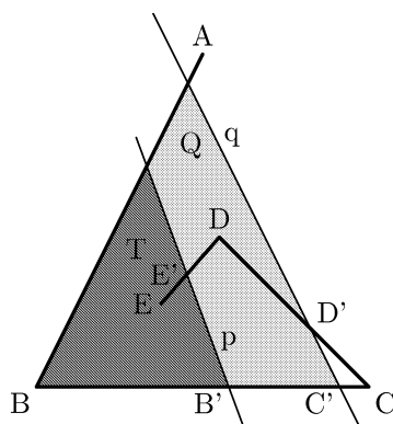
Figure 4: The triangle ABC , the point D inside it, the triangle T and quadrilateral Q , and the forced position of the point E .
