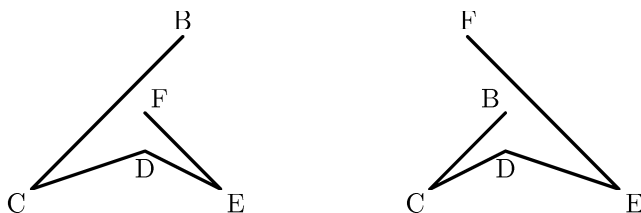
Figure 8: The cases that the point F is in \psi or \chi are symmetric.
