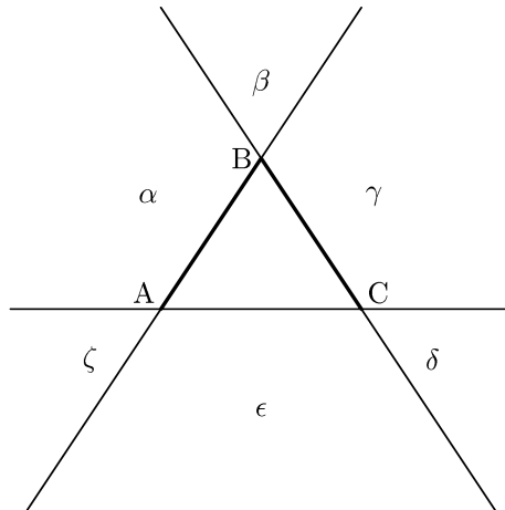
Figure 11: The six regions \alpha, \beta, \gamma, \delta, \epsilon, \zeta where the vertex D can lie.
