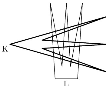
Figure 2: A k -gon K and an l -gon L with k(l - 1) intersections for even k and odd l .
