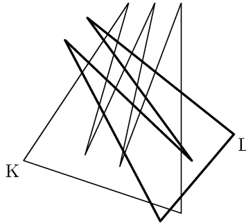
Figure 3: A k -gon K and an l -gon L with kl - k - l + 3 intersections for both k and l odd.
