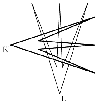
Figure 1: A k -gon K and an l -gon L with kl intersections for k and l both even.
