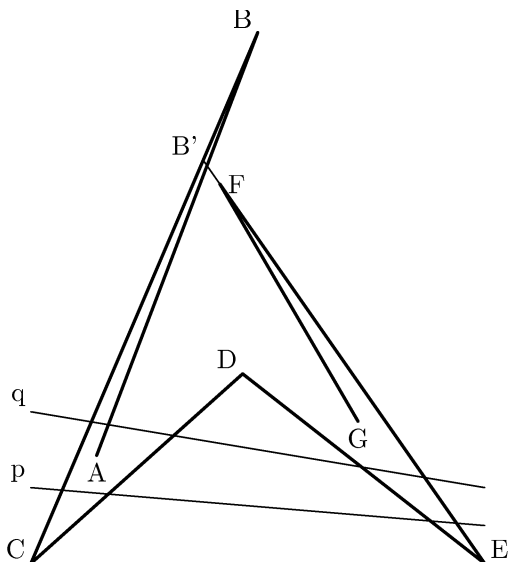
Figure 9: The segments p and q and the triangle T' .
