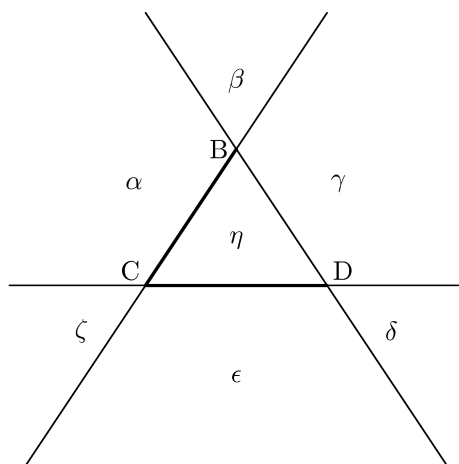
Figure 5: The seven regions \alpha, \beta, \gamma, \delta, \epsilon, \zeta and \eta in which the lines BC, CD and BD split the plane.
