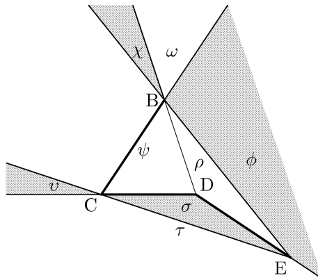
Figure 7: The regions \sigma , \tau , v , \phi , \chi , \psi , \rho and \omega ; the regions \sigma , v , \phi and \chi are marked by gray.
