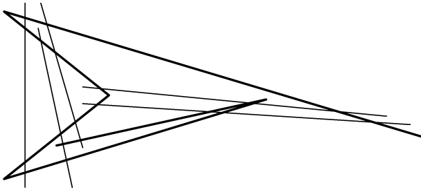
Figure 10: A path of length five and a set of five non-intersecting segments such that their non-intersection graph is a perfect matching.
