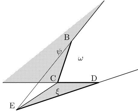
Figure 6: The regions \xi , \psi and \omega ; \xi and \psi are marked by gray.
